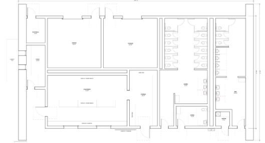
Schematic Plan
