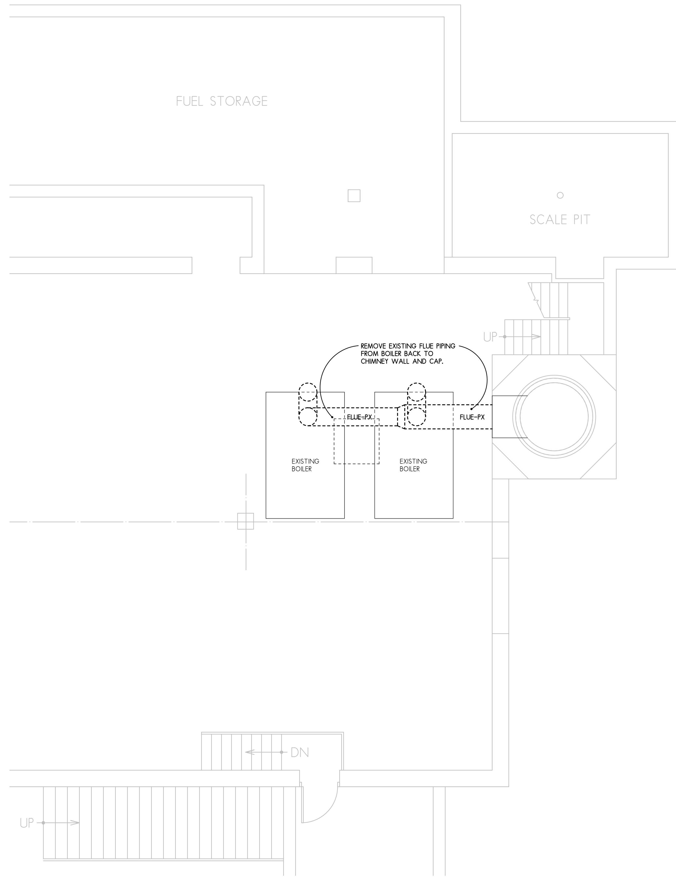
1 BOILER ROOM HVAC DEMOLITION PLAN SCALE: 1/4" = 1'-0"
