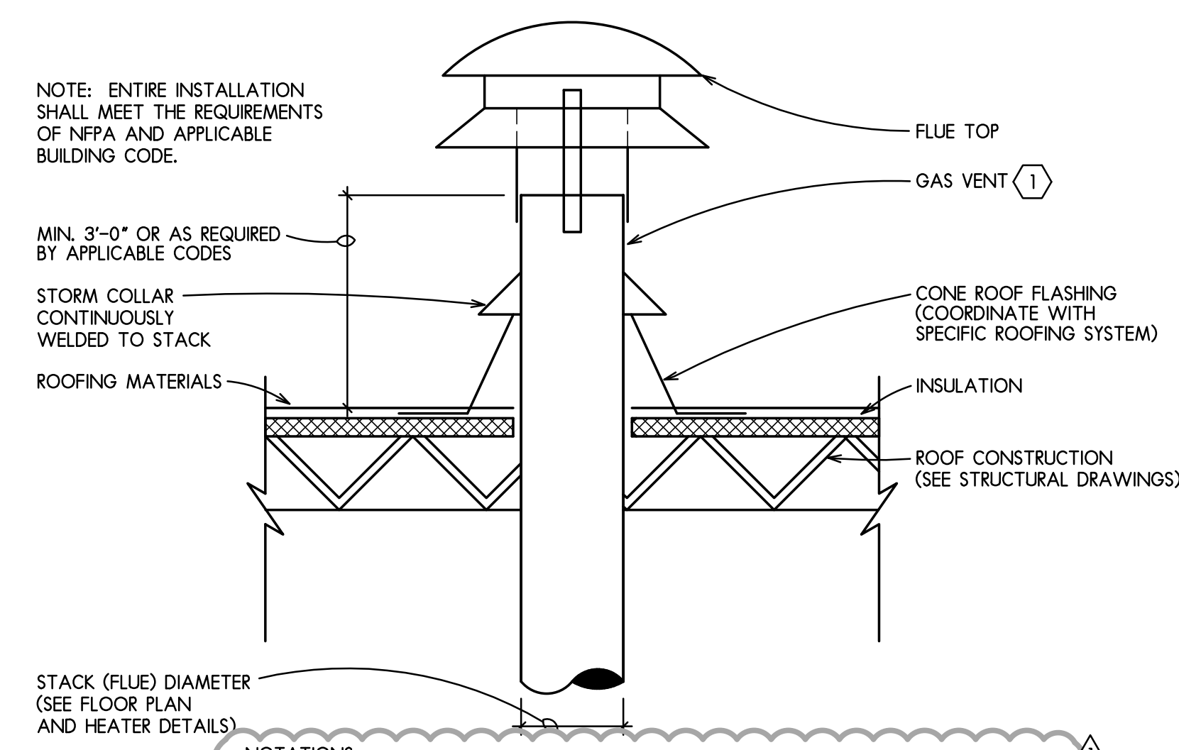
3 FLUE THRU ROOF NO SCALE
