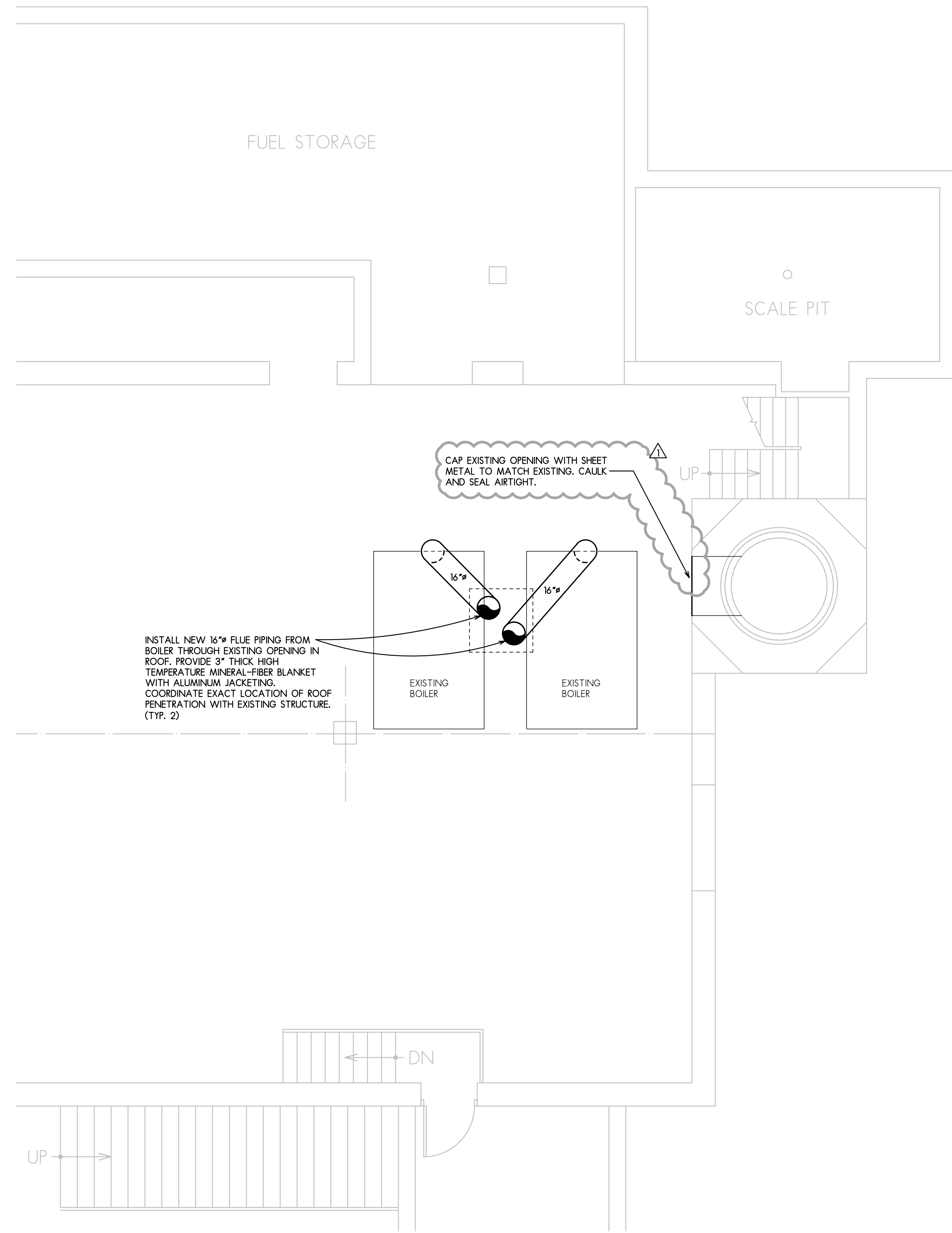
2 BOILER ROOM HVAC NEW WORK PLAN SCALE: 1/4" = 1'-0"
