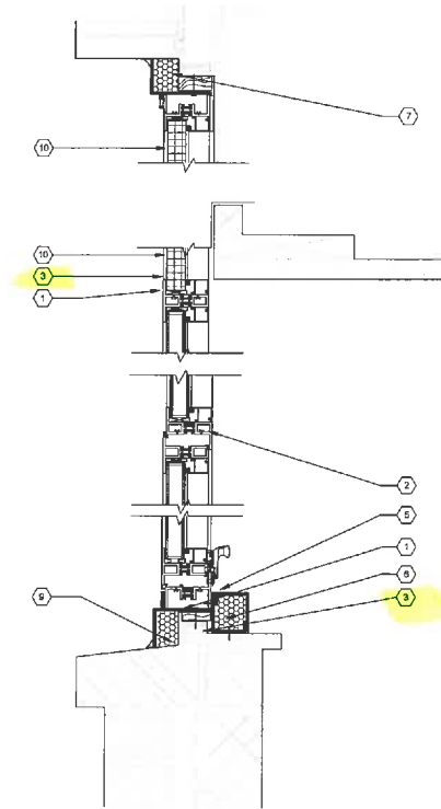
1 SECTION DETAIL - TYPICAL 3" = 1'-0"
