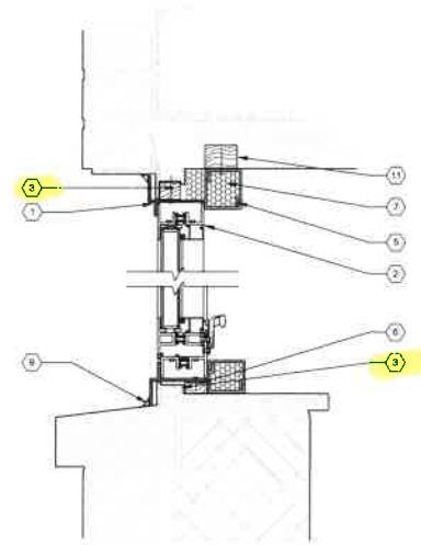
4 SECTION DETAIL - WINDOW TYPE D 3" = 1'-0"
