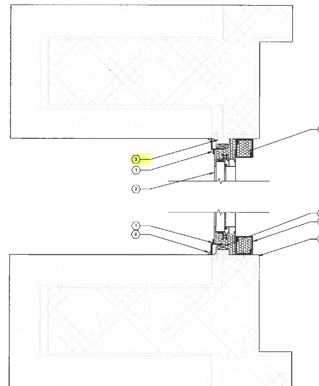
2 WINDOW REPLACEMENT JAMB DETAIL 3" = 1'-0"
