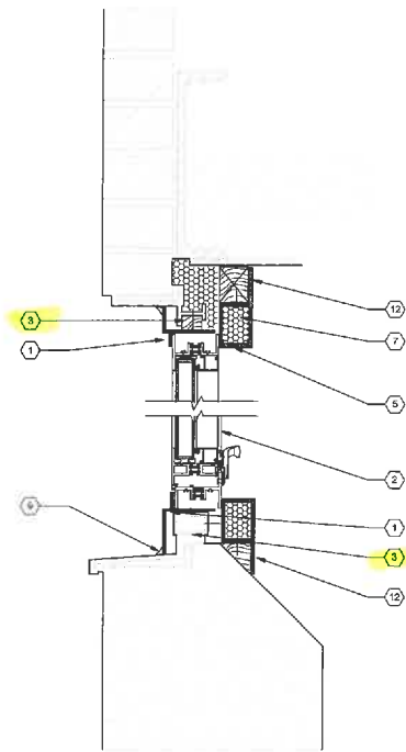
3 SECTION DETAIL - BASEMENT 3" = 1'-0"
