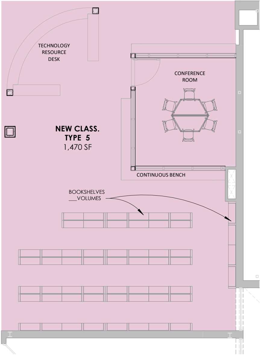
1- TYPE 5
