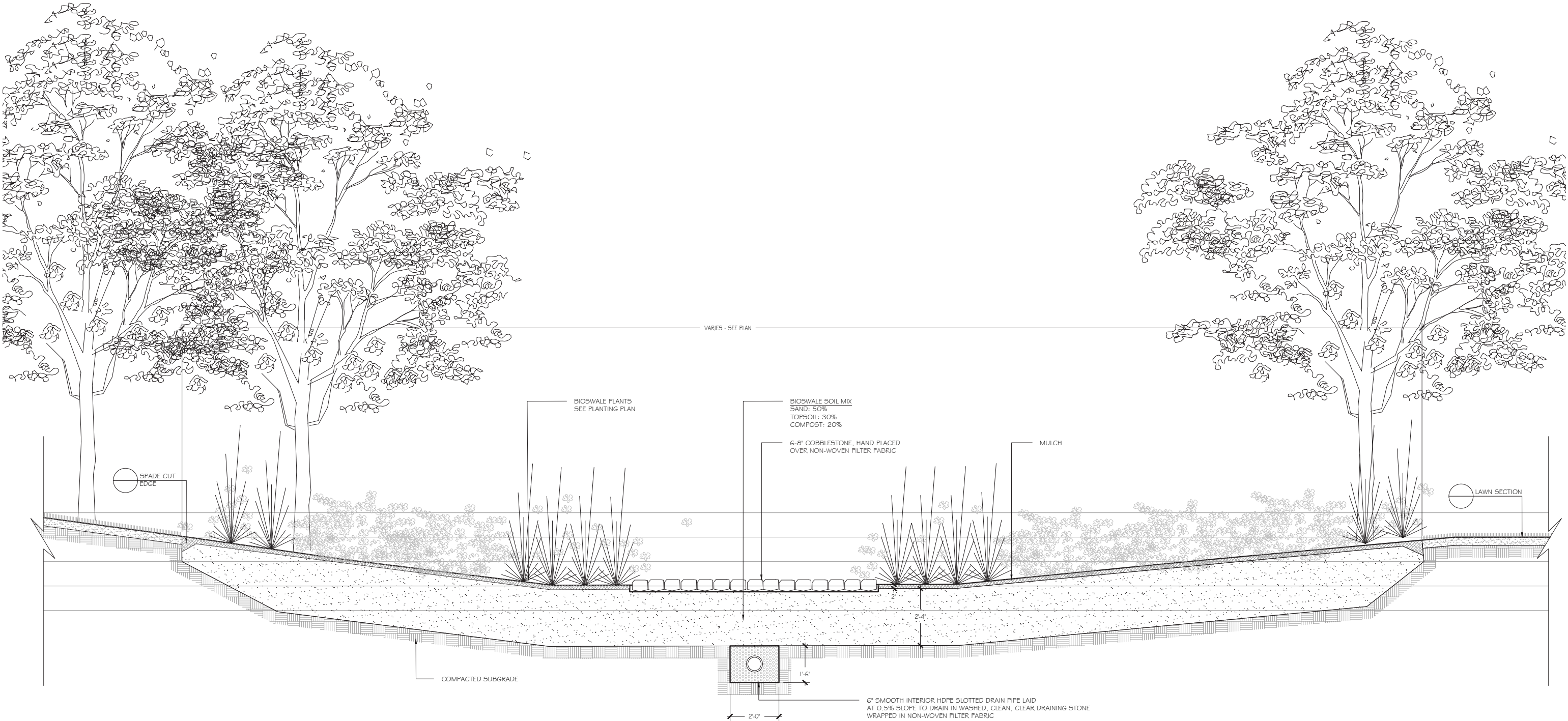
BIOSWALE SECTION 1/2"=1'-0"
