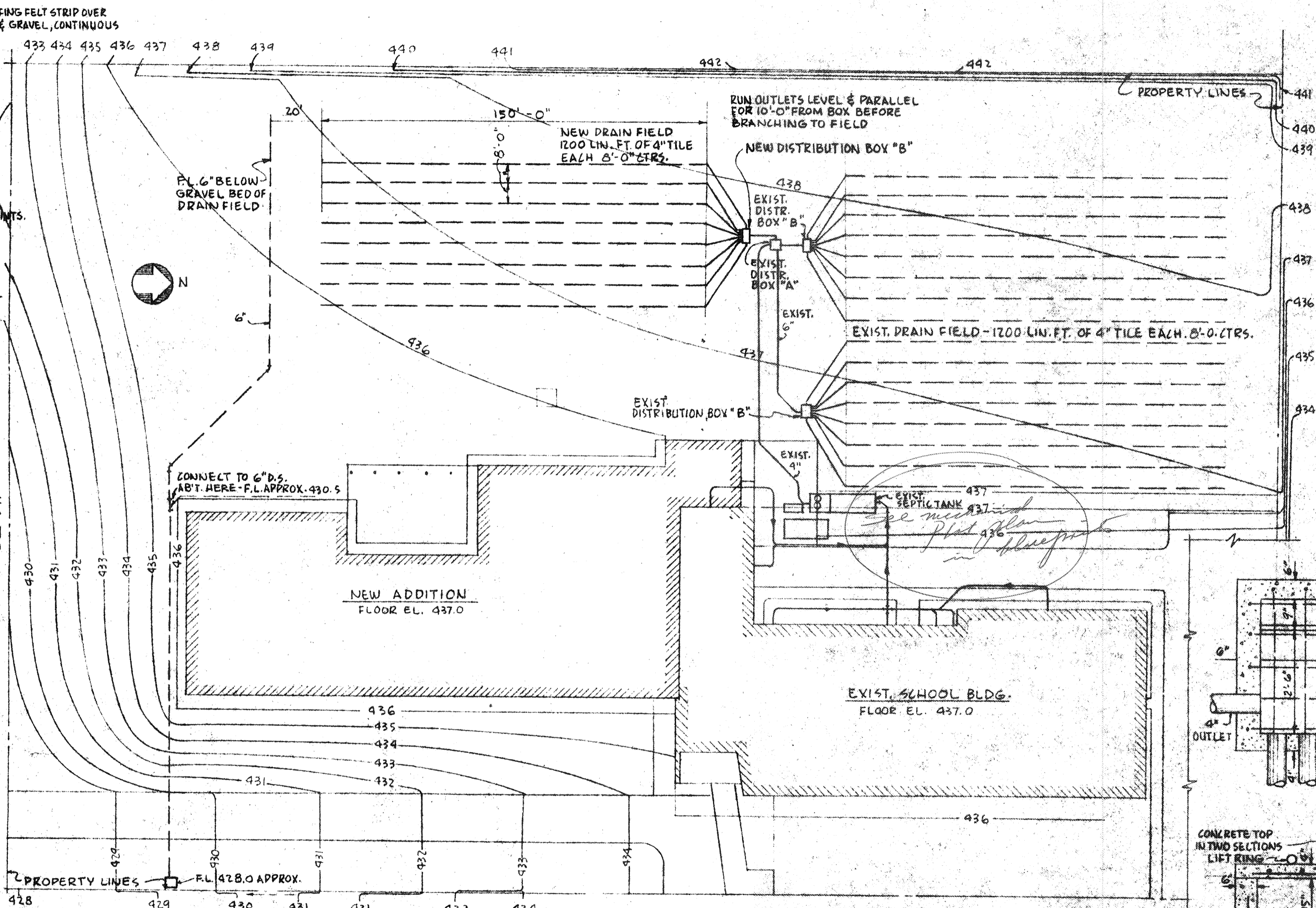
THIRD AVENUE SOUTH PLOT PLAN SCALE: 1/32" = 1'-0" FINISH GRADES SHOWN
