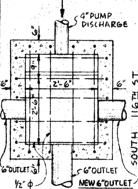
PLAN
