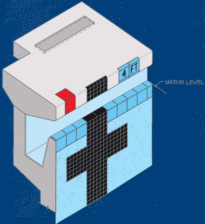
Cantilever Gutter
